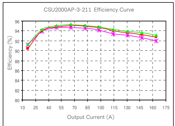
Figure 48: CSU2000AP-3-211 Efficiency Curve @ 25°C 180Vac 230Vac 264Vac Loading: I_{o,max} = 10\% I_{o,max} increment to I_{o,max}
