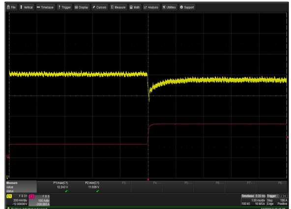
Figure 46: CSU2000AP-3-211 Transient Response - V_o Deviation 40% to 100% load change 0.5A/ \mu s slew rate V_{in} = 230V_{ac} Ch 1: V_o Ch 2: I_o
