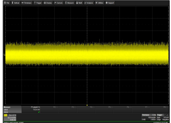
Figure 44: CSU2000AP-3-211 Ripple and Noise Measurement V_{in} = 230V_{ac} Load: I_o = 163.9A I_{SB} = 3.5A Ch 1: V_o
