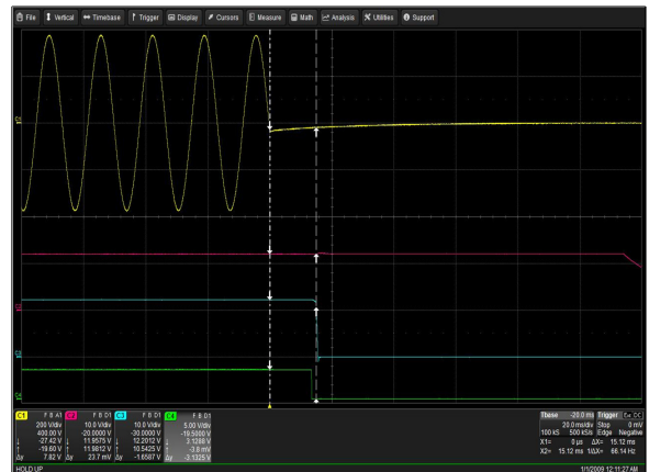
Figure 16: CSU2000AP-3-111 Hold-Up Time Vin = 264Vac Load: I O = 163.9A I SB = 3.5A Ch 1: AC Mains Ch 2: V SW Ch 3: V O Ch 4: PWOK
