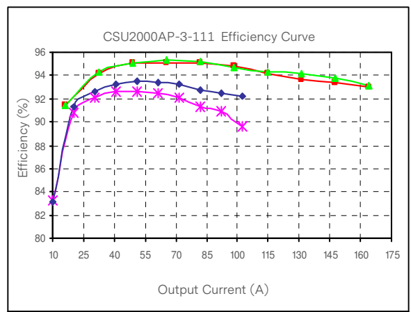
Figure 24: CSU2000AP-3-111 Efficiency Curve @ 25°C Loading: I_{o,max} increment to I_{o,max}
