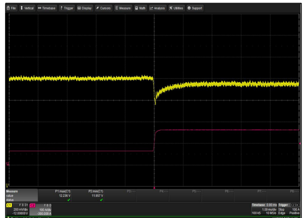
Figure 22: CSU2000AP-3-111 Transient Response - V_o Deviation 40% to 100% load change 0.5A/ \mu S slew rate Vin = 230Vac Ch 1: V_o Ch 2: I_o
