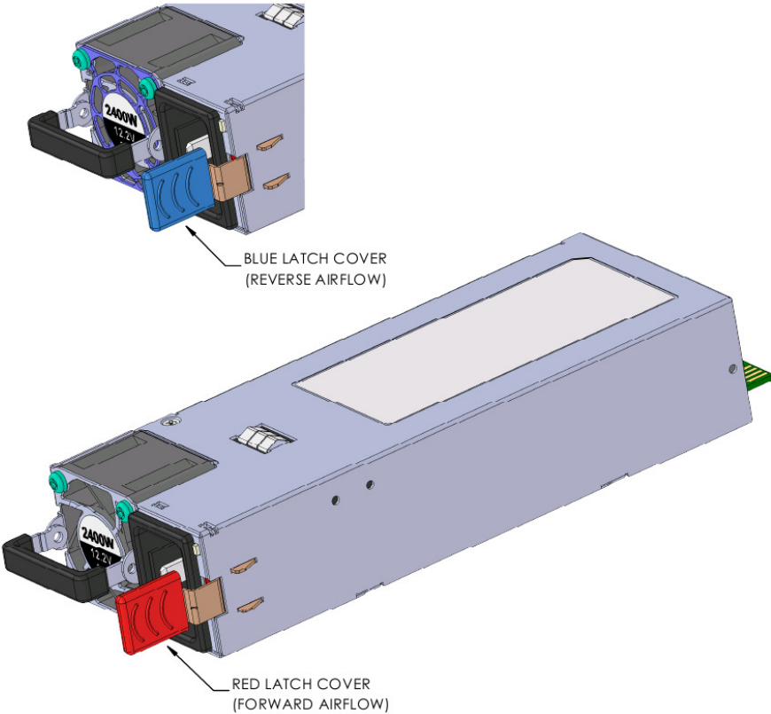
Mechanical Outlines CSU2000AP-3-200/-211 (unit: mm)
