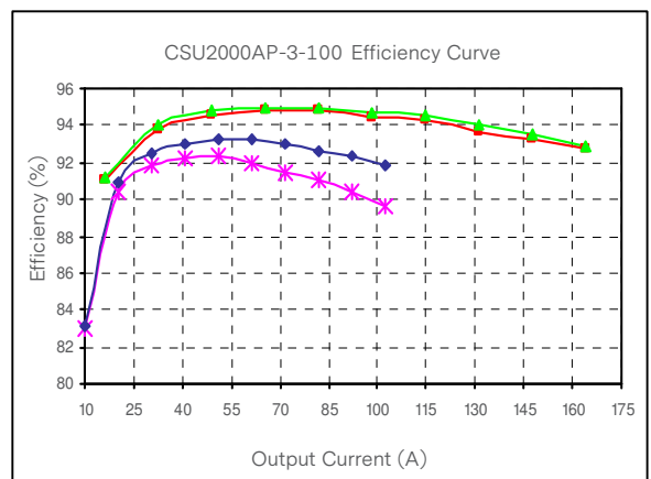
Figure 12: CSU2000AP-3-100 Efficiency Curve @ 25°C Loading: I o,min = 10% I o,max increment to I o,max
