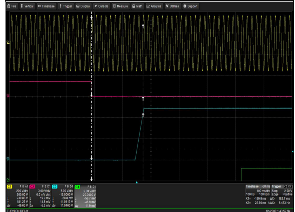
Figure 38: CSU2000AP-3-211 Turn-On Delay via PSON Vin = 180Vac Load: I O = 163.9A I SB = 3.5A Ch 1: AC Mains Ch 2: PSON Ch 3: V O Ch 4: PWOK
