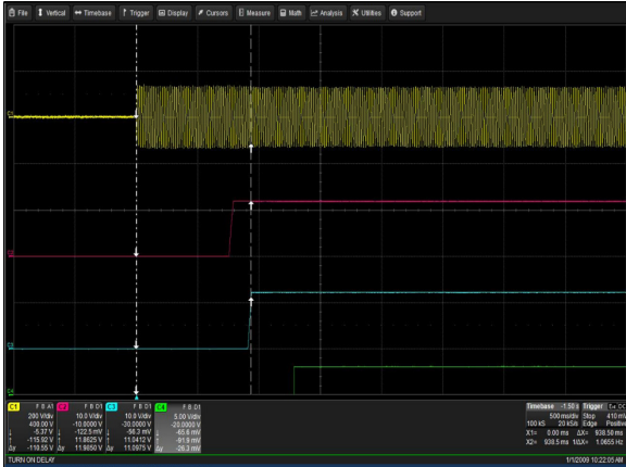
Figure 13: CSU2000AP-3-111 Turn-On Delay via AC Mains Vin = 90Vac Load: I O = 102.5A I SB = 3.5A Ch 1: AC Mains Ch 2: V SW Ch 3: V O Ch 4: PWOK
