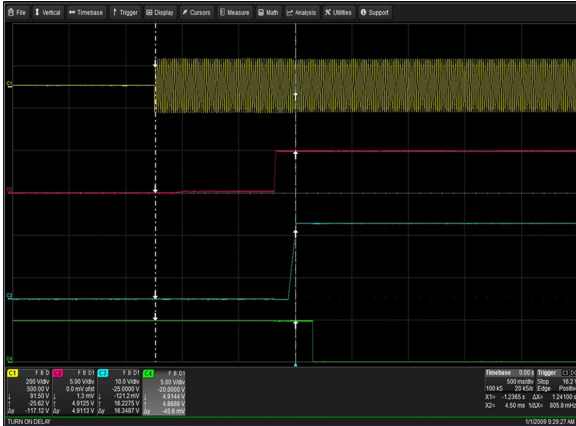
Figure 15: LCM30008-T Turn-on delay via AC mains Vin = 90Vac Load: lo = 83.3A (18V), Isb = 2A Ch 1: Vin Ch 2: Vsb Ch 3: Vo Ch 4: G_DCOK_C
