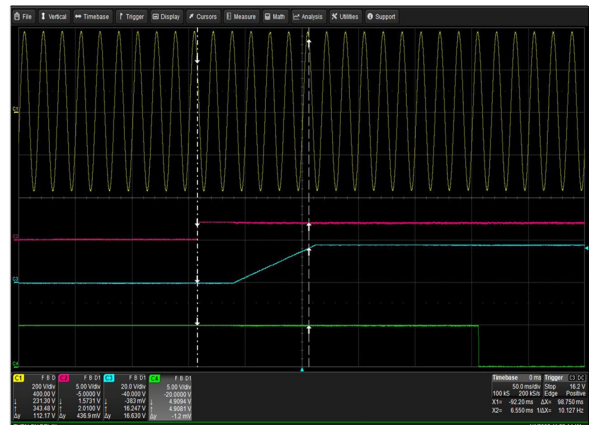
Figure 18: LCM30008-T Turn-on delay via INH_EN Vin = 264Vac Load: lo = 166.7A (18V), Isb = 2A Ch 1: Vin Ch 2: INH_EN Ch 3: Vo Ch 4: G_DCOK_C
