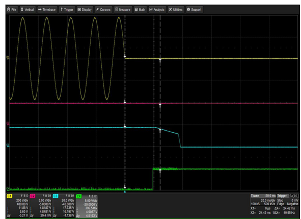
Figure 20: LCM30008-T Hold-up Time Vin = 264Vac Load: lo = 166.7A (18V), Isb = 2A Ch 1: Vin Ch 2: Vsb Ch 3: Vo Ch 4: G_DCOK_C
