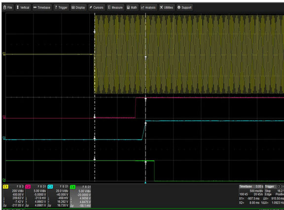
Figure 17: LCM30008-T Turn-on delay via AC mains Vin = 264Vac Load: lo = 166.7A (18V), Isb = 2A Ch 1: Vin Ch 2: Vsb Ch 3: Vo Ch 4: G_DCOK_C
